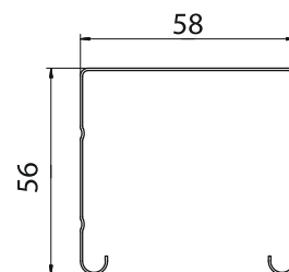
HEAD RAIL
